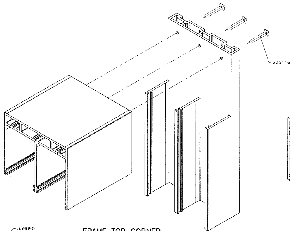
FRAME TOP CORNER (2 TRACK FRAME)
