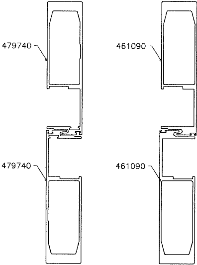
STANDARD INTERLOCKS
